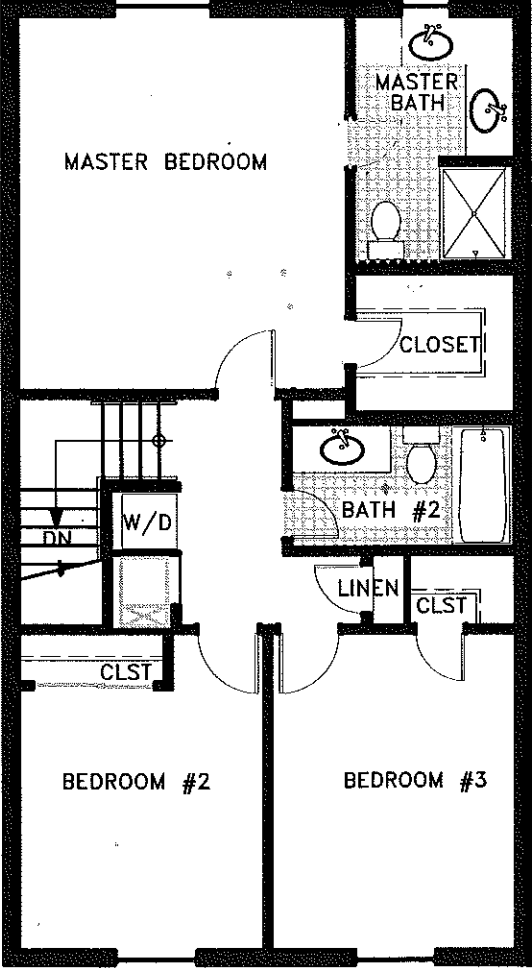
Type L-2A Three Bedroom Two and Half Bath Townhouse
