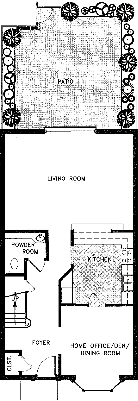
Type L-2A Three Bedroom Two and Half Bath Townhouse
